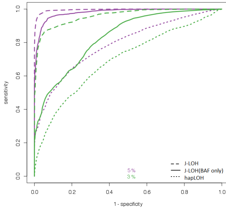
Figure S3: Comparison of ROCs between hapLOH and J-LOH at tumor purities 3% and 5%. We first classify existence of any aberration state by applying different thresholds to the posterior probability of being normal to obtain the ROC. Since hapLOH uses only the BAF information, we ran J-LOH first with both BAF and LRR and then with BAF inputs only.
