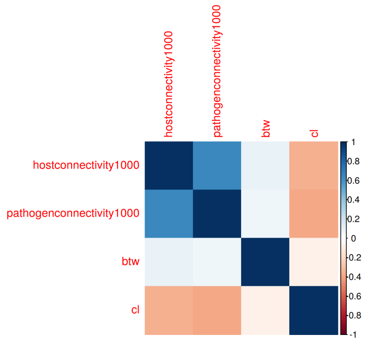
Fig 1. Correlations between different covariates in the statistical model: the two connectivity measures and the the two network summary statistics betweenness (btw) and closeness (cl).
