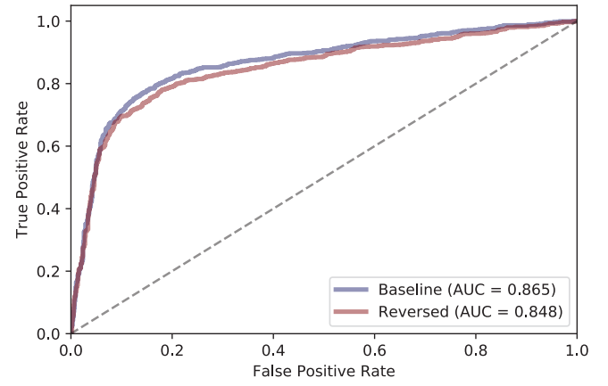
ROC curve for HepG2 sample
