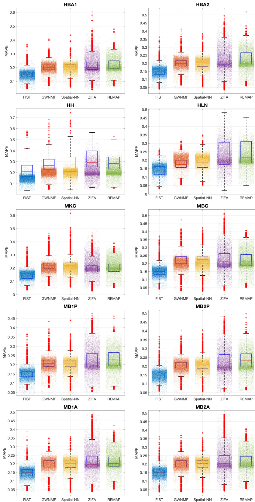
Gene-wise imputation performance by MAPE. The performances on the imputations of each gene are shown as box plots. The MAPE of every gene slice is denoted by one dot. The performance of each method is shown in each colored box plot.
