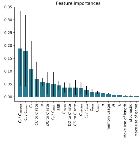
(c) Importance of features for clusters on 50% performance. (d) Importance of features for clusters based on k means algorithm.
