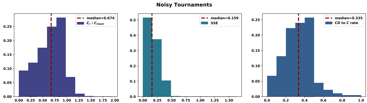
Figure 7: Distributions of C_r/C_{\text{mean}} , SSE and CD to C ratio for the winners of noisy tournaments.
