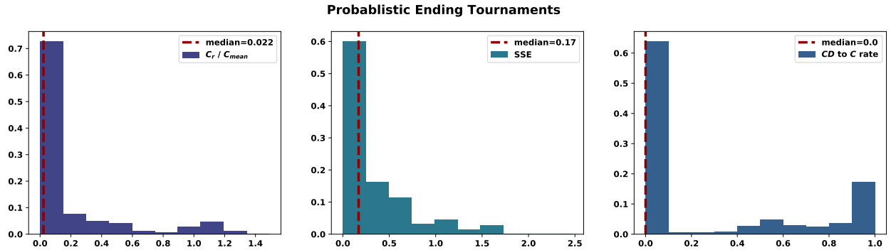
Figure 9: Distributions of C_r/C_{\text{mean}} , SSE and CD to C rate for the winners of probabilistic ending tournaments.
