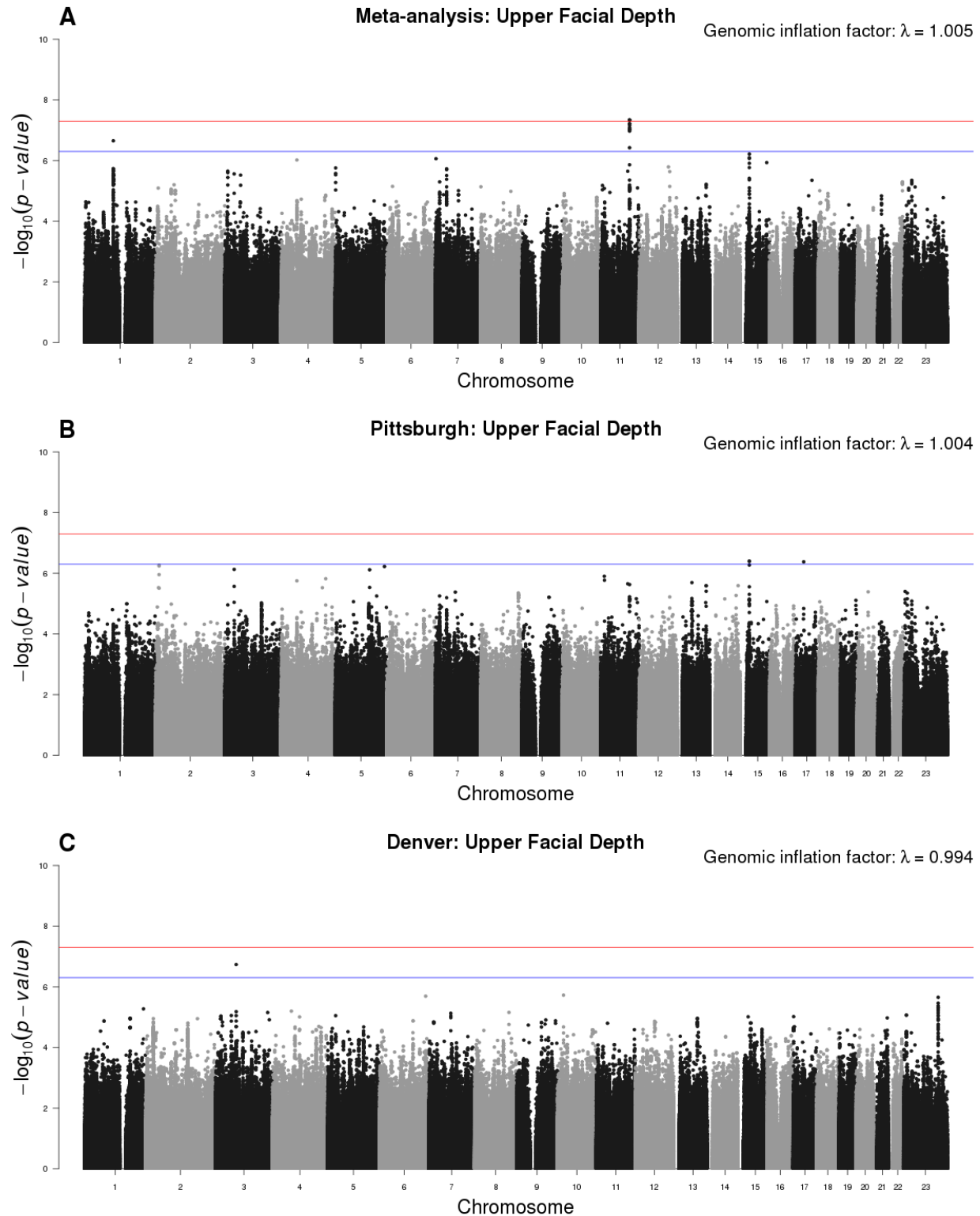
S2 Fig. Manhattan plots for upper facial depth. (A) meta-analysis results, (B) Pittsburgh sample results, and (C) Denver sample results. Lines for p-value thresholds set at 5 \times 10^{-8} for genome-wide significance and 5 \times 10^{-7} for suggestive significance
