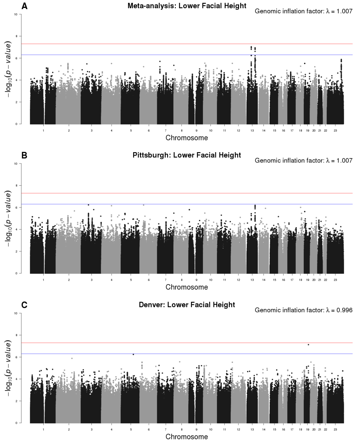
S7 Fig. Manhattan plots for lower facial height. (A) meta-analysis results, (B) Pittsburgh sample results, and (C) Denver sample results. Lines for p-value thresholds set at 5 \times 10^{-8} for genome-wide significance and 5 \times 10^{-7} for suggestive significance.
