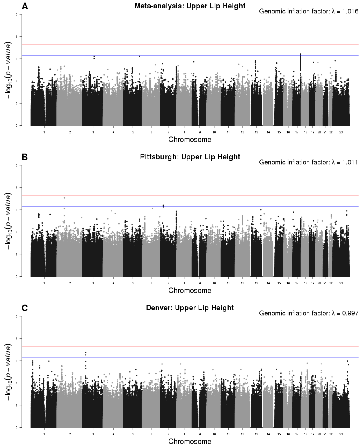
S19 Fig. Manhattan plots for upper lip height. (A) meta-analysis results, (B) Pittsburgh sample results, and (C) Denver sample results. Lines for p-value thresholds set at 5 \times 10^{-8} for genome-wide significance and 5 \times 10^{-7} for suggestive significance.
