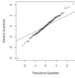
B Normal Q-Q Plot
