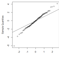
C Normal Q-Q Plot
