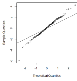
A Normal Q-Q Plot
