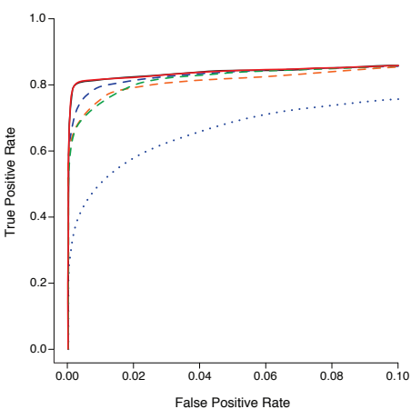
(A) SNP-Level Methods (Sparse Traits)
