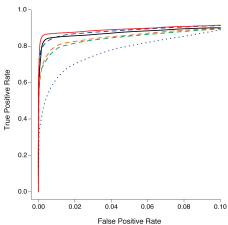
(A) SNP-Level Methods (Sparse Traits)
