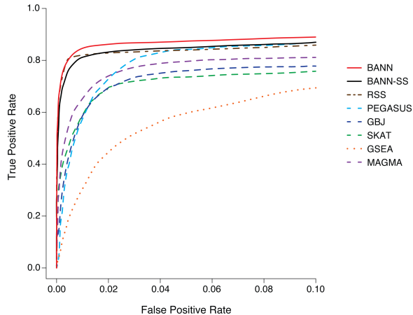
(B) SNP-Set Methods (Sparse Traits)
