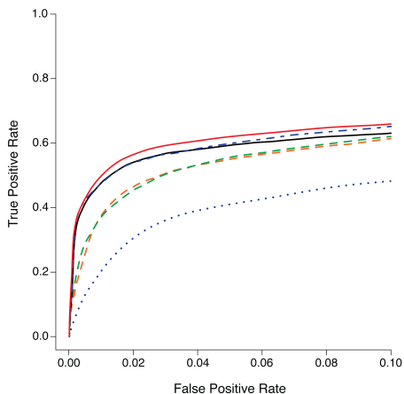
(C) SNP-Level Methods (Polygenic Traits)
