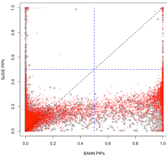
(C) SNP-Level Methods (Polygenic Traits)
