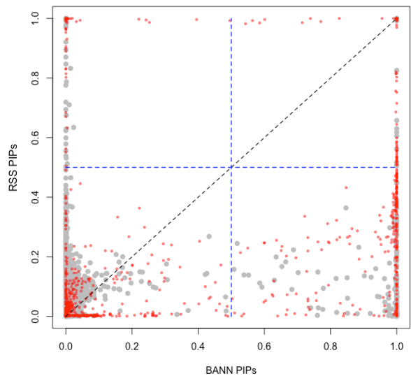
(B) SNP-Set Methods (Sparse Traits)
