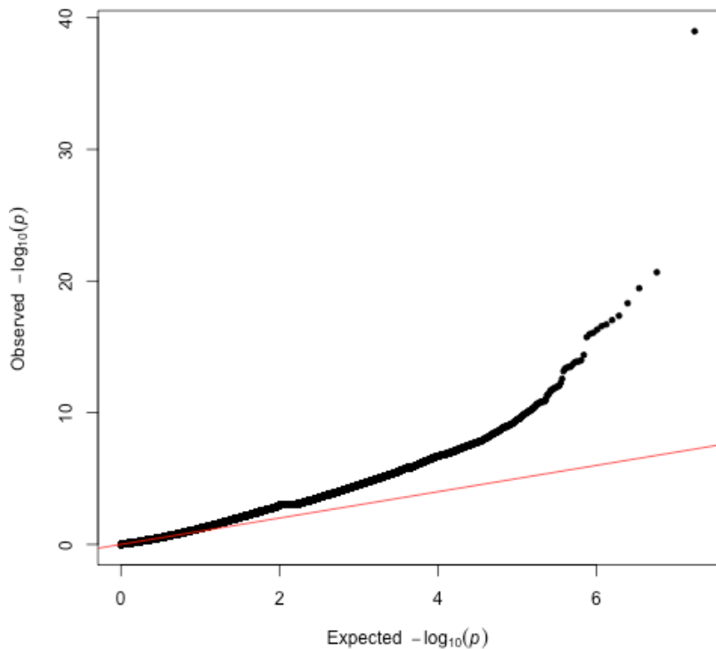
S10 Fig: QQ plot of the selection scan result of the whole genome SNPs by Relate.
