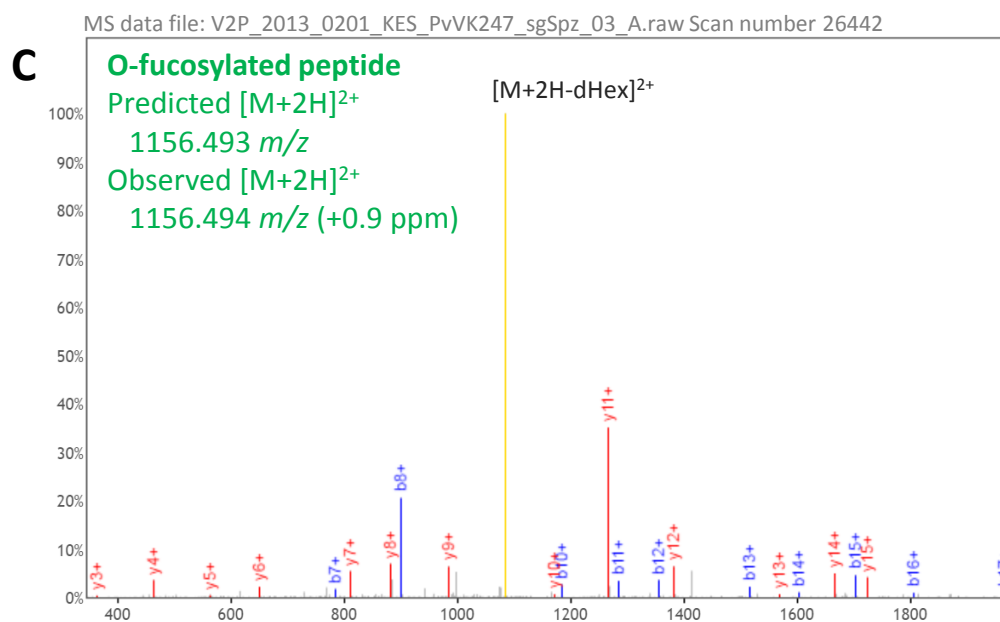
S8 Fig. Evidence for glycosylation of TRAP in P. vivax VK247 salivary gland sporozoites. (A) Representative extracted ion chromatograms (XIC) of the doubly-charged ions of the TRAP peptide VANGPWPDPWTACSVTCGK from P. vivax VK247 salivary gland sporozoites. The largest chromatographic peak (green) was produced by a species with a mass matching the peptide plus a deoxyhexose, which we presume to be O-fucose. The unmodified peptide was observed co-eluting with the putatively-fucosylated species, consistent with loss of the gas-phase-labile modification due to collision-induced dissociation (CID) within the mass analyzer source. Unlike for CSP (S5 Fig and S6 Fig), the unmodified peptide was not observed except arising from neutral loss of the glycan, suggesting that all or nearly all of the TRAP present in the sample was glycosylated. Representative collision-induced dissociation (CID) fragmentation spectra of the unmodified (B) and glycosylated (C) peptides confirmed the peptide sequence. CID of the peptide lacking O-fucose (B) provided confirmation of the assignments of the fragment spectra obtained from the O-fucosylated species (C). Fragment ions are annotated as b-ions (blue) and y-ions (red). The unfragmented peptide is designated M (yellow) with addition of protons (H) and neutral loss of deoxyhexose (dHex). Fucose is a deoxyhexose. Fragmentation spectra of the O-fucosylated peptide showed that the dominant product of CID fragmentation was the intact peptide that had lost the O-linked glycan. No peptide fragment spectra were observed with the O-fucose glycan intact, so the location of the glycan could not be confirmed, but based on the presence of the O-fucosylation motif, we presume that the Thr of CSVTCG was modified.
