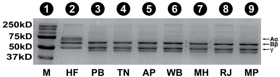
Fig. S3. Fibrinogenolytic activities of N. naja venoms from distinct locations across India.
