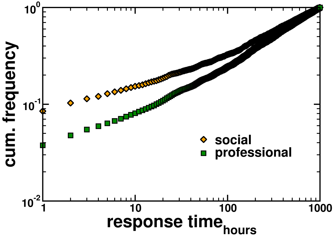
Figure S3: We display the frequency distribution of response times for different types of ties utilizing email transmissions among more than 500 MBA students over a 2-year period of time. Specifically, we only accounted for time intervals of < 1,000 hours. We conclude that social ties have shorter response times than professional ties.
