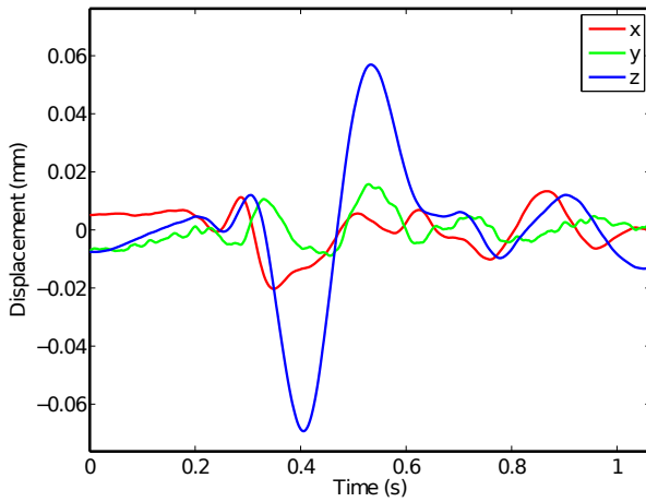
Fig. S3. Ballistocardiograms computed using tracking data from (A) the 1.5 T and (B) the 3 T experiments (see Fig. 5 for results obtained at 7 T). In each case, the effect appears most strongly as a shift along the head-feet direction.
