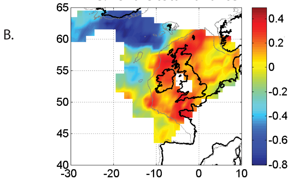
Eigenvector 2 Calanus (1948-2007) 11.28% of the total variance
