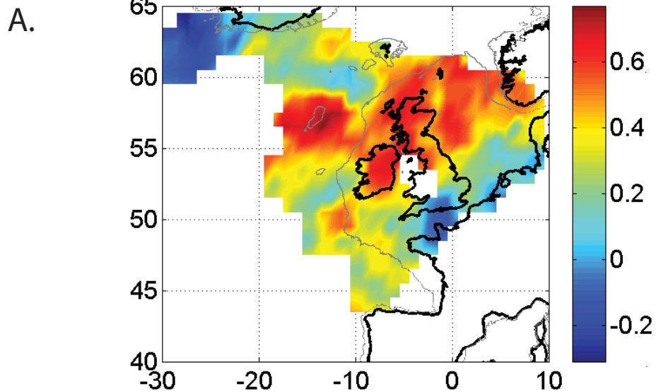
Eigenvector 2 Calanus (1948-2007) 11.28% of the total variance
