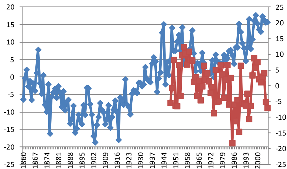
In red Second PC Calanus and in blue second PC SST
