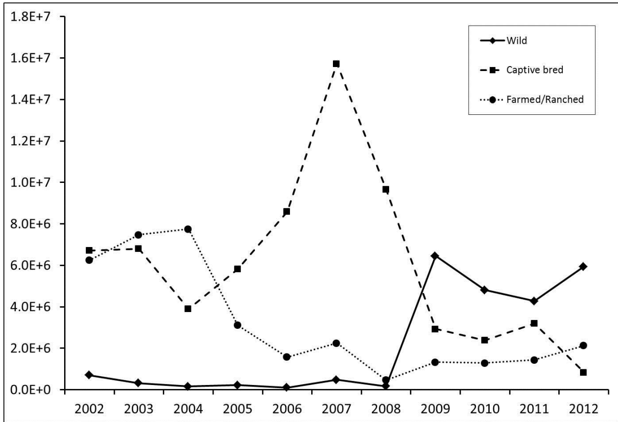
Supplemental Fig. S1. Total number of exported turtles (y-axis) from 2002-2012 (x-axis) partitioned by the source of turtles.
