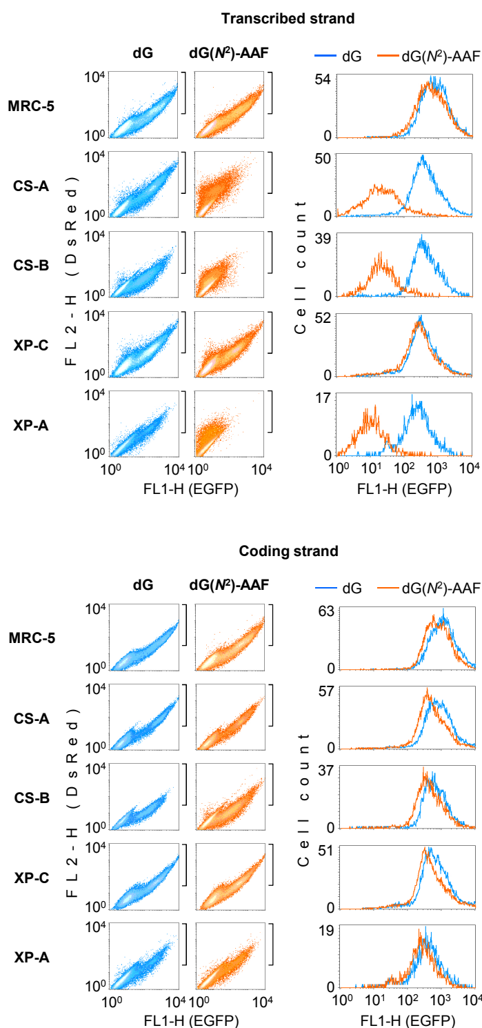
Supporting Figure 5. Host cell reactivation in human cell lines of the specified nucleotide excision repair complementation groups (CS-A, CS-B, XP-C and XP-A) and in the repair proficient cell line (MRC-5). The expression constructs contained synthetic oligonucleotides with a unique dG( N^2 )-AAF (amber colors) or dG (blue colors) in the specified DNA strand. Dot density plots obtained in a representative experiment and the corresponding overlaid fluorescence distribution plots. Extended data for the experiment shown in Figure 3.
