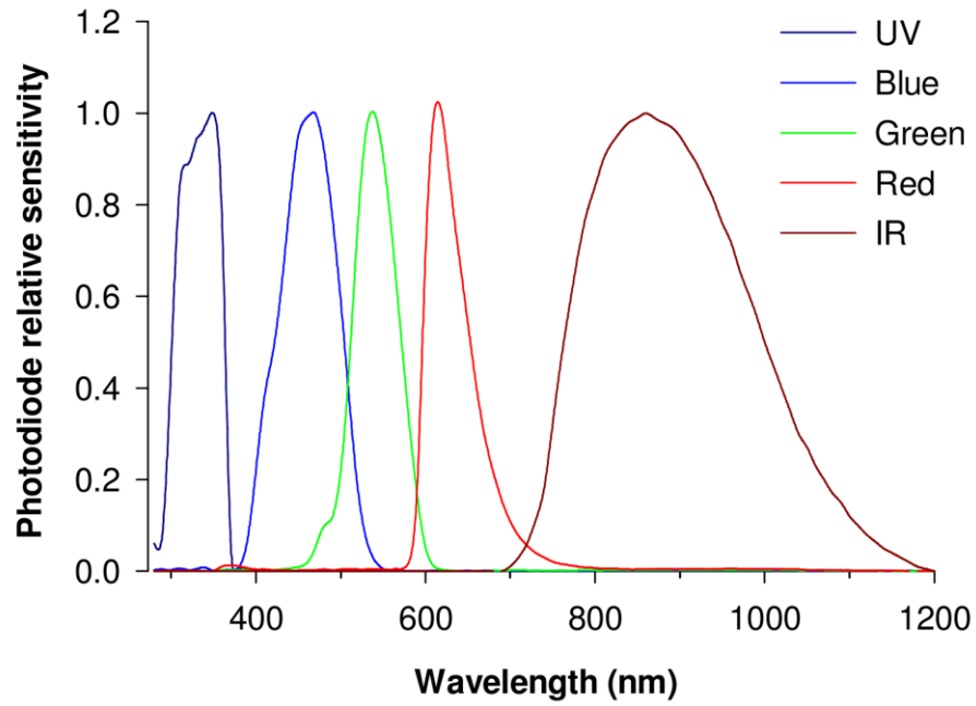
Figure S1. Relative spectral sensitivity of the LightWatcher's photodiodes. The device (Lighwatcher) contains 5 photodiodes with peak sensitivities around: IR (860 nm), red (620 nm), green (540 nm), blue (460 nm) and UV lights (350 nm). This device was used to monitor continuously individual spectral light exposure during the study.
