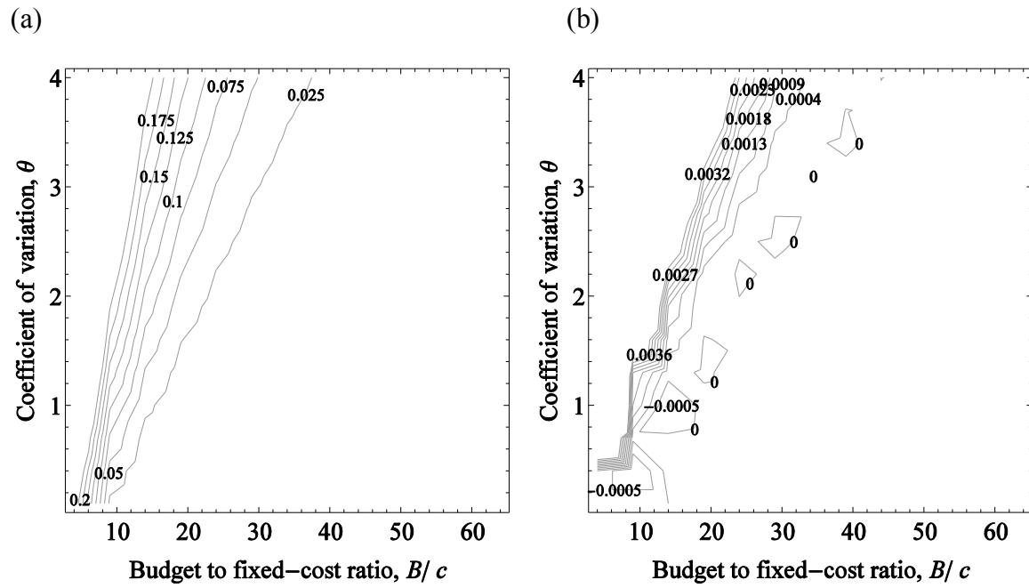
Figure S3. Value of objective function for objective 1. (a) expected probability of failed-detection E[Q] for exact solution, (b) difference in expected probability of failed-detection E[Q] for exact and approximate solutions. c' = 0.5 .
