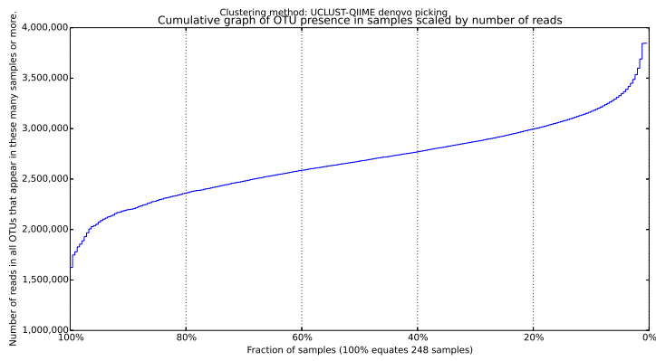
(b) UCLUST clustering method
