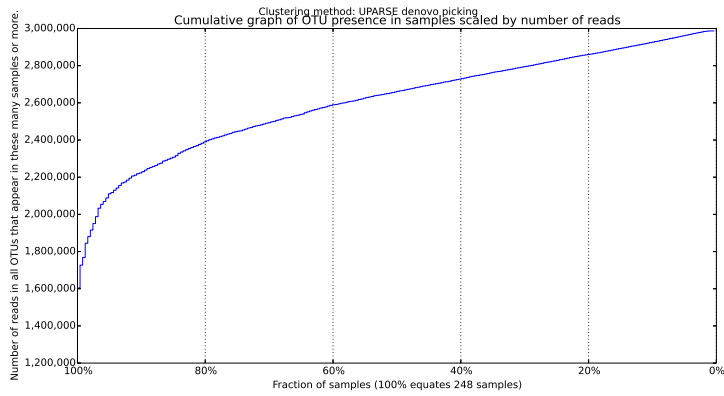
(a) UPARSE clustering method
