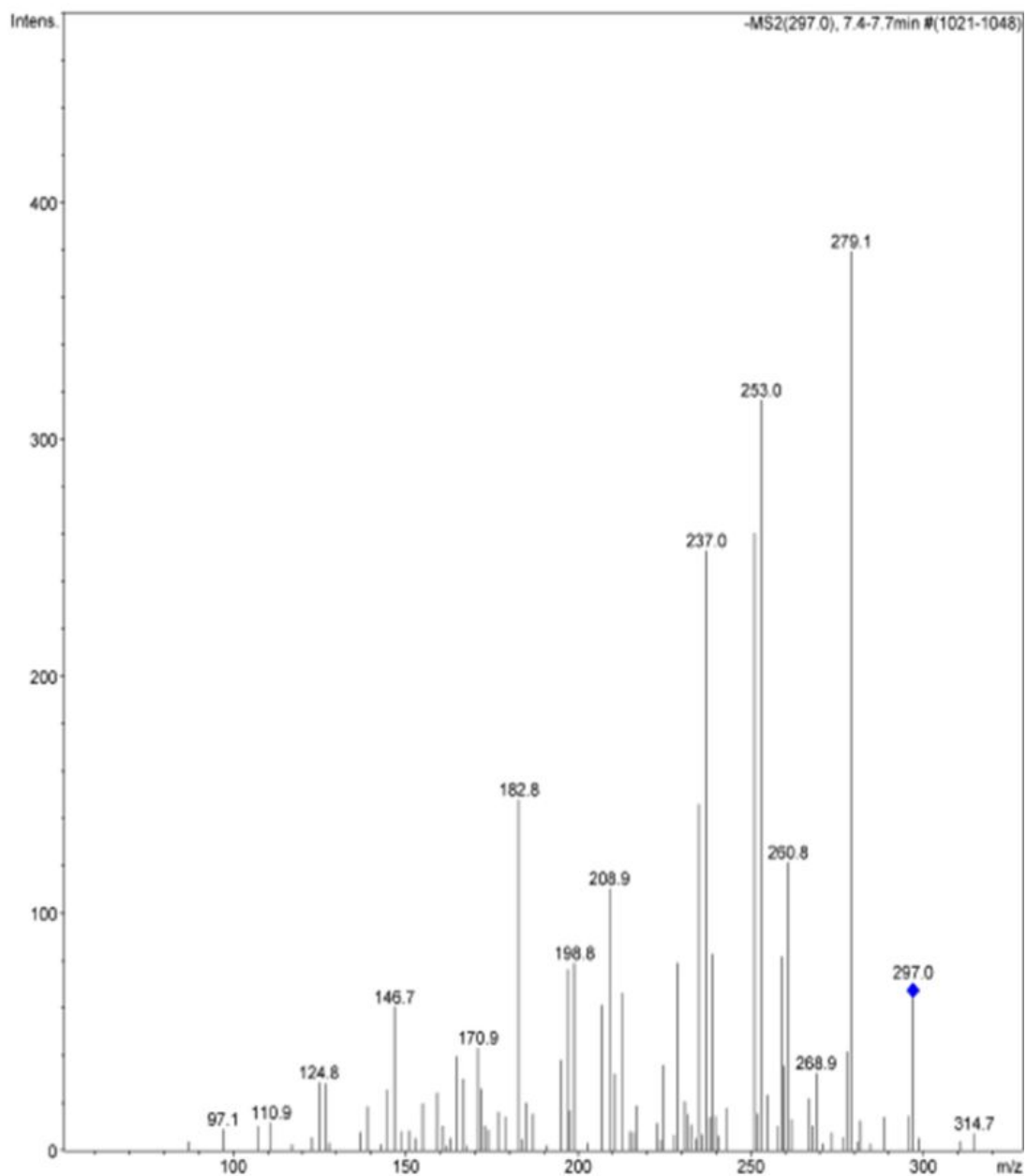
S3 Fig. Fragmentation pattern of 18-hydroxyoleic acid. The compound was analyzed with an Agilent 1100 series LCMSD ion trap XCT Plus system. The fragmentation was generated by using a collision energy of 20 volts and negative ionization mode.
