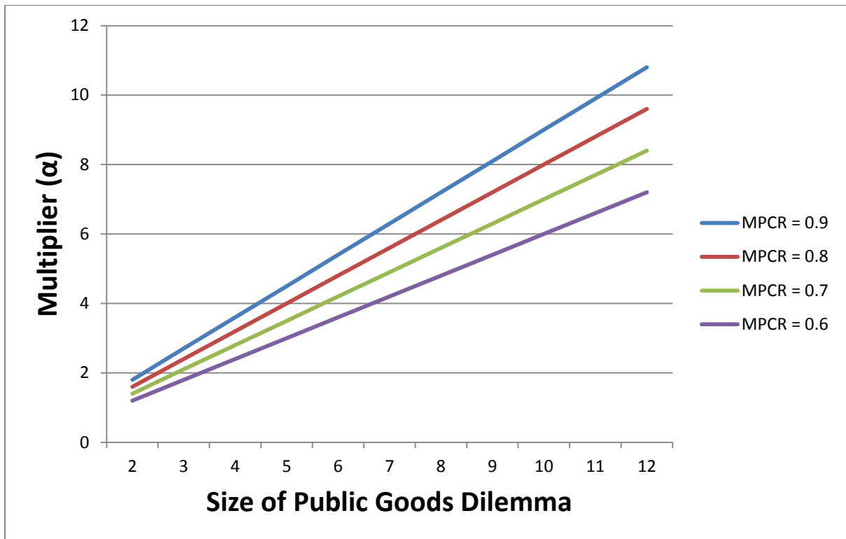
S2 Figure. Multiplier values by different sizes of public goods dilemma and different Marginal Per Capita Return values. MPCR values are always between 0 and 1, but for a 2-person public goods dilemma, the MPCR must remain about .5, so we have shown four values to cover the range of .5 to 1.
