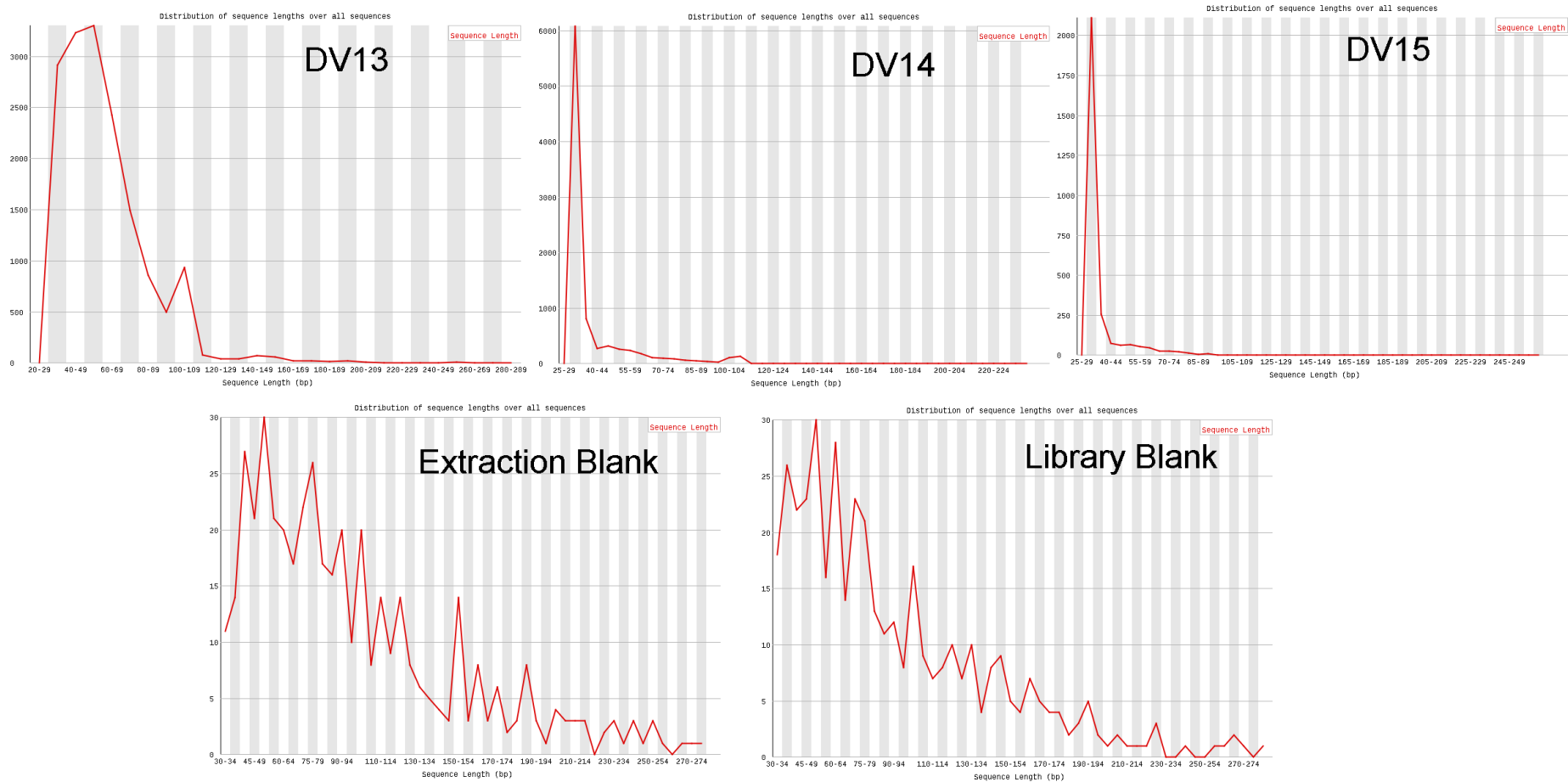
Figure S2. Read length distribution. Distribution of reads mapping to hg19. Negative controls show an excess of unspecific mapping reads under 30bp.
