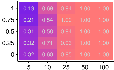
C_2 causes C_1
