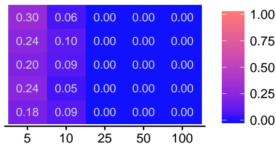
C_1 causes C_2
