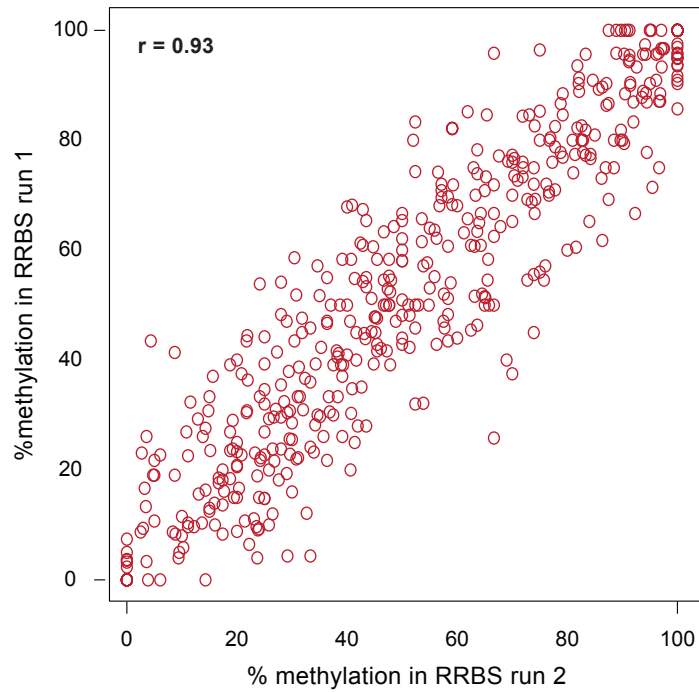
Fig S2. Methylation levels at outlier sites are highly correlated in two independent RRBS runs. Scatter plot showing methylation levels (5methylcytosine as a proportion of all cytosine) of outlier sites in twin pair 2 in two independent RRBS runs.
