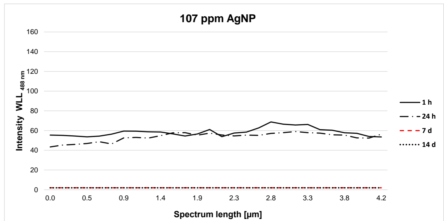
S2 Fig. Changes of the chlorophyll fluorescence spectrum of the A. lobatus control cells and cells treated with AgNP concentrations at every hour/day of the experiment.
