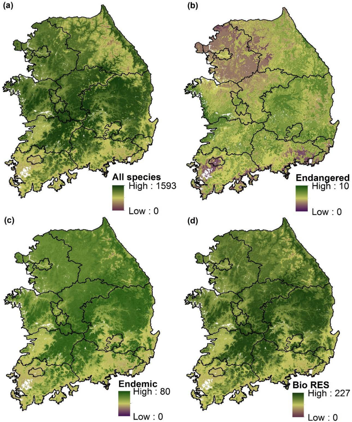
S1 Fig. Combined species richness maps from MARS SDM for each group category for South Korea: (a) All species, (b) Endangered species, (c) Endemic species, and (d) Biological resource species. The values in legend represent the number of species: greener areas have higher plant species richness in each group category.
