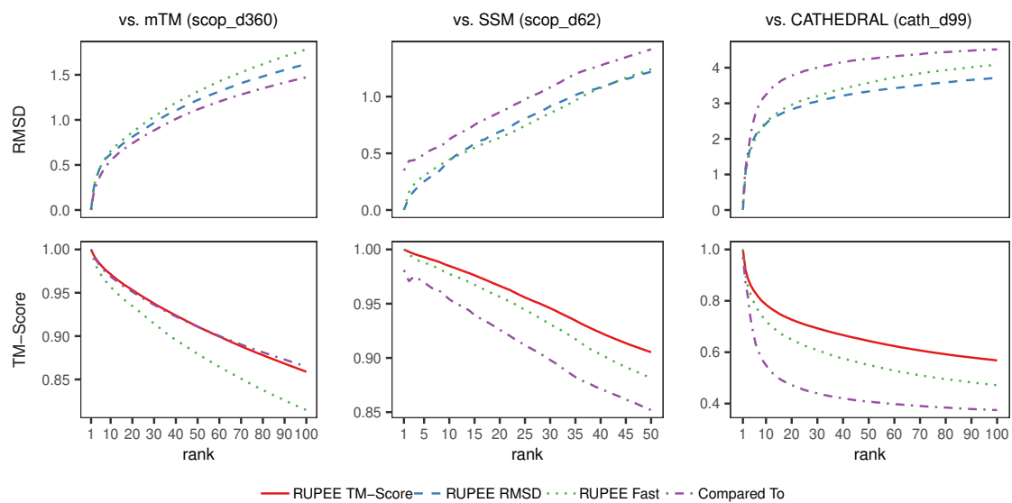
Figure 1: Scoring from CE pairwise alignments for RUPEE fast, RUPEE top-aligned sorted by TM-Score, and RUPEE top-aligned sorted by RMSD
