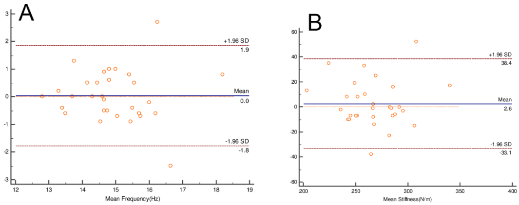
S2 Fig. Examples Bland-Altman plots for MyotonPRO measurement of dominant rectus femoris tone(A) and stiffness(B) of healthy males. 95% limits of agreement and mean difference marked with dotted(--) and solid (—)lines.
