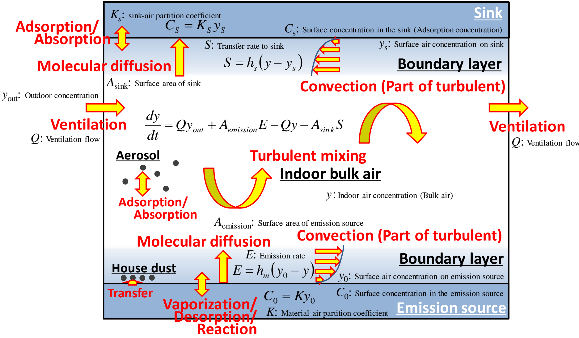
S1 Figure. Schematic representation of semi-volatile organic compounds (SVOCs) in an indoor environment (Detailed version).
