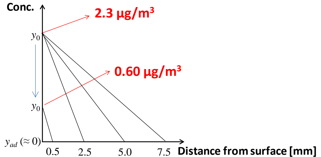
S5 Figure. Schematic diagram of surface concentration and concentration gradient for samples A, B, and C.
