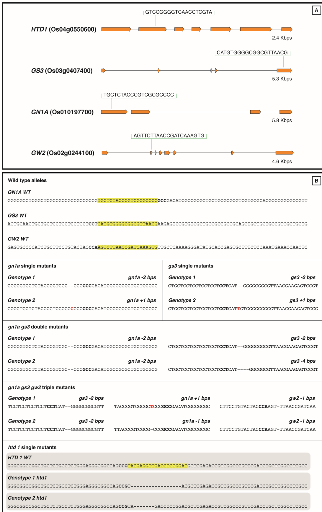
Supplemental Figure S2: A) exon – intron structure of target loci, gRNA sequences are reported for each locus, B) mutant genotypes considered in this study, gRNAs are highlighted in yellow, PAM sequence in bold
