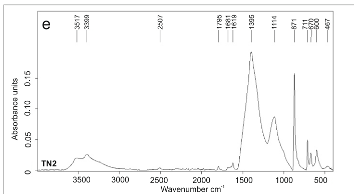
S3 Fig. Infrared spectra and thermal analysis curves. Representative ATR-FTIR spectra and TG-DSC-DTG curves of samples PAL2 (a,b), T76L (c,d) and TN2 (e,f).
