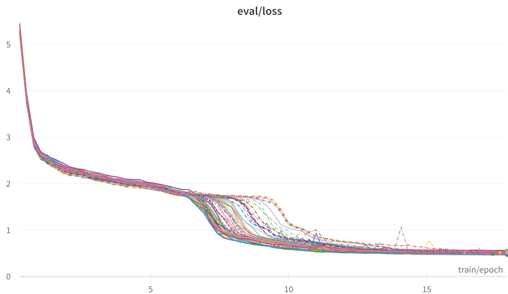
S1 Fig. Eval loss during pre-training. Eval loss during pre-training, each line corresponds to one of 60 models.
