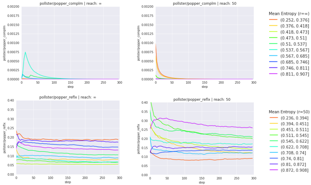
S2 Fig. Evolution of Popper metrics complementarity and reflexivity during self-training. Left: inferentially closed pre-training corpora (reach= \infty ); right: inferentially incomplete pre-training corpora (reach=50). Metric evolutions are aggregated over all agents whose belief systems display a similar joint entropy (cf. bins to the very right).
