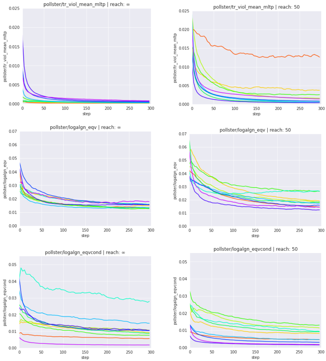
S3 Fig. Evolution of Consistency Metrics transitivity violation ratio , equivalence , and antecedent equivalence during self-training. Left: inferentially closed pre-training corpora (reach= \infty ); right: inferentially incomplete pre-training corpora (reach=50). Metric evolutions are aggregated over all agents whose belief systems display a similar joint entropy (cf. legends in S2 Fig ).
