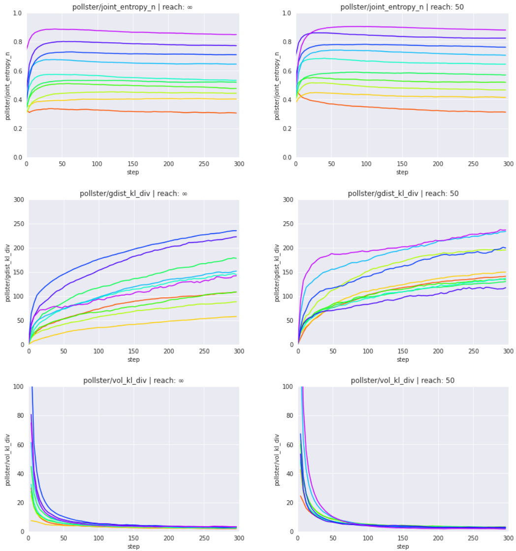
S4 Fig. Global dynamics (evolution of joint entropy, global distance, volatility) during self-training. Left: inferentially closed pre-training corpora (reach= \infty ); right: inferentially incomplete pre-training corpora (reach=50). Metric evolutions are aggregated over all agents whose belief systems display a similar joint entropy (cf. legends in S2 Fig ).
