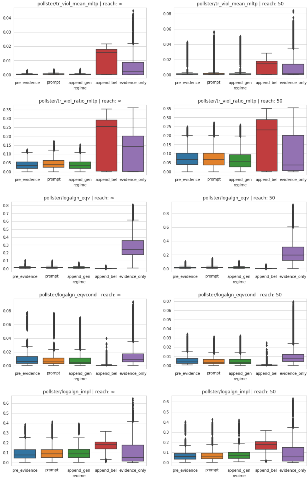
S12 Fig. Comparison of Consistency Metrics before and after evidence introduction. Comparison of Consistency Metrics before and after evidence introduction for different evidence introduction regimes. Left column: inferentially closed pre-training corpora (reach= \infty ); right column: inferentially incomplete pre-training corpora (reach=50).
