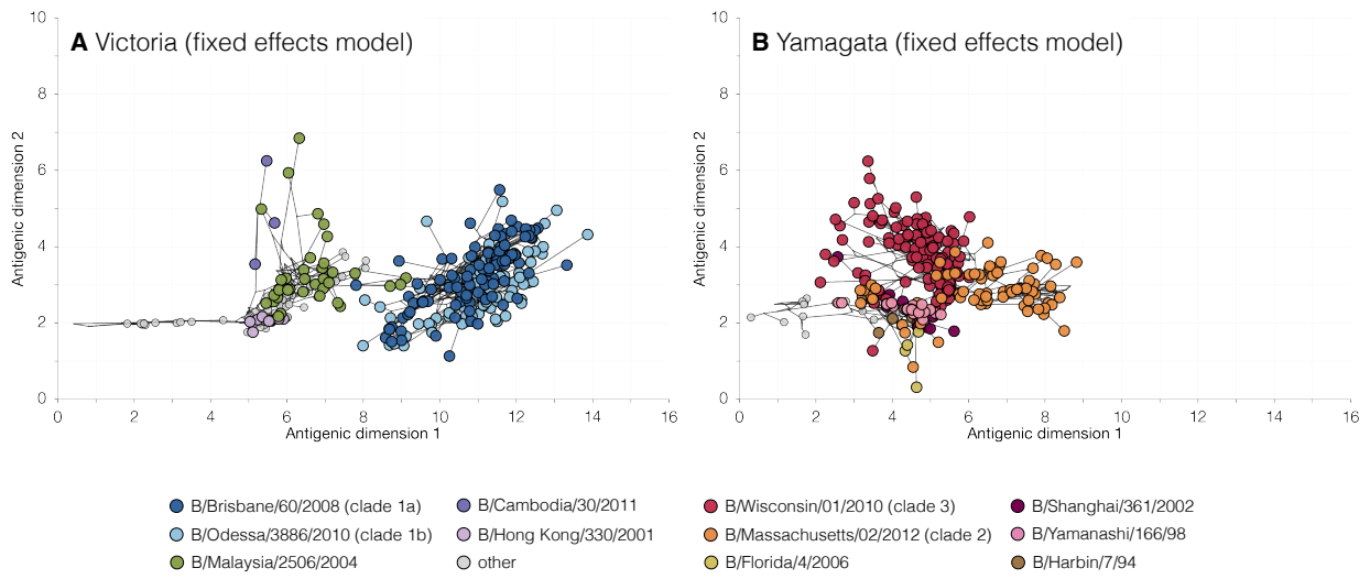
S4 Fig. Antigenic and genetic evolutionary relationships of (A) Victoria-lineage and (B) Yamagata-lineage influenza B viruses inferred using a BMDS model with fixed serum potencies and virus avidities. See Fig 4 legend for further details.
