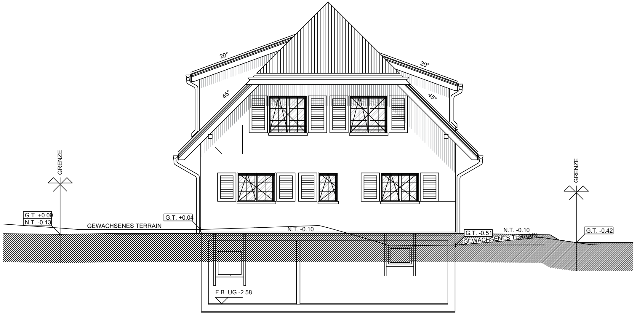
NORD-WEST FASSADE
