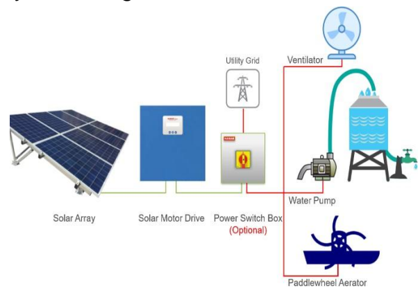
System Diagram
