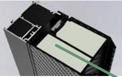
HYBRID OF ALUMINUM FRAME AND CARBON STRUCTURED FIBER GLASS COMPOSITE
