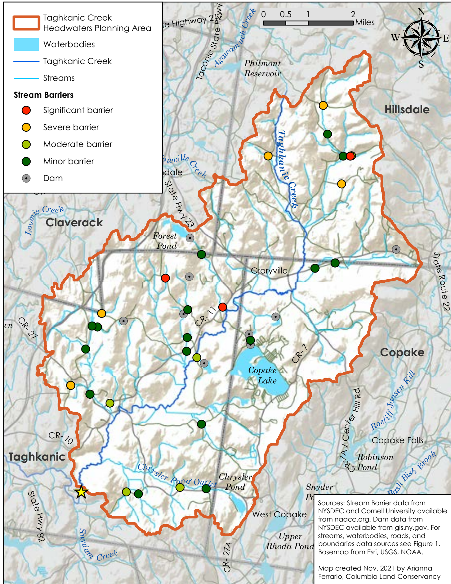
Figure 13. Stream Barriers
