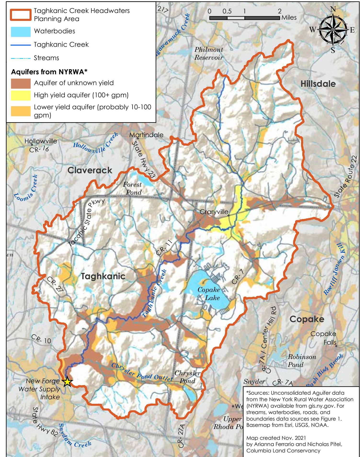
Figure 12. Aquifers
