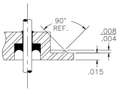
PIN 14 GRD. DETAIL SCALE: 8:1
