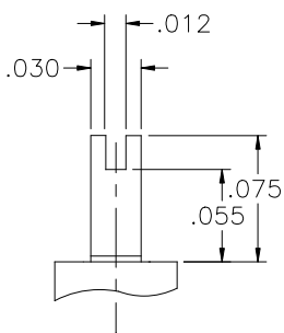
CENTER MOUNT DETAIL
