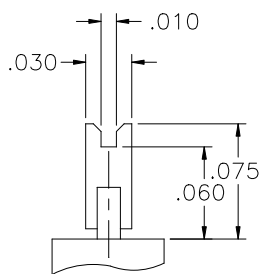
OUTSIDE MOUNT DETAIL
