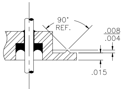
PIN 7 GRD. DETAIL SCALE: 8:1
