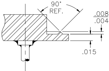
PIN 3,5,10 & 12 GRD. DETAIL SCALE: 8:1
